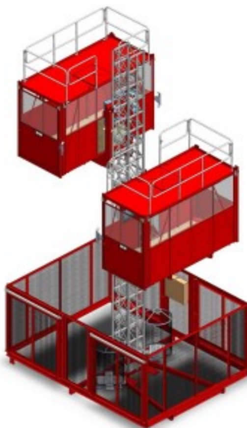
TWIN HOIST
