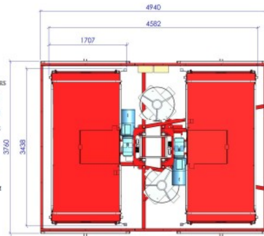
TWIN HOIST
